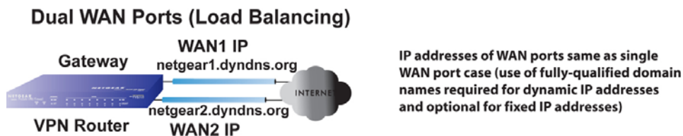
Figure B-8 Load Balancing for Dual Gateway WAN Ports
