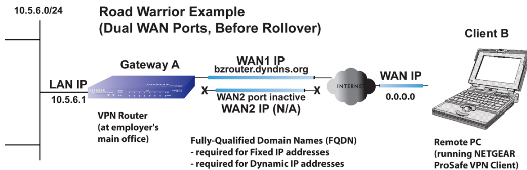
Figure B-10 Road Warrior, Dual Gateway WAN Ports
