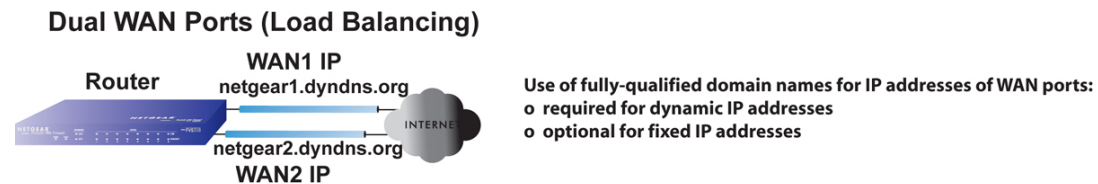
Figure B-3 Load Balancing Case for Firewalls with Dual WAN Ports
