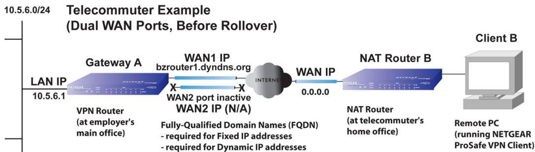
Figure B-18 Telecommuter, Dual WAN Ports, Before Rollover
