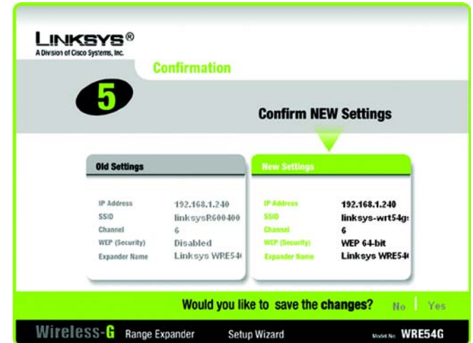
Figure 5-13: Confirmation Screen
