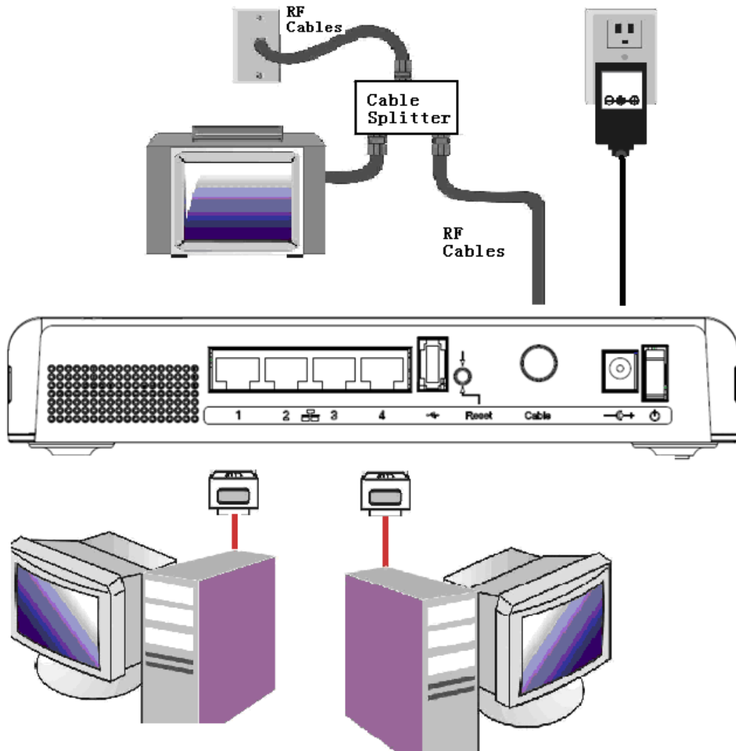
Fig.3: Multiple-PC Connection
