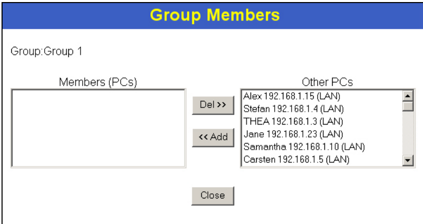
Figure 37: Group Members
