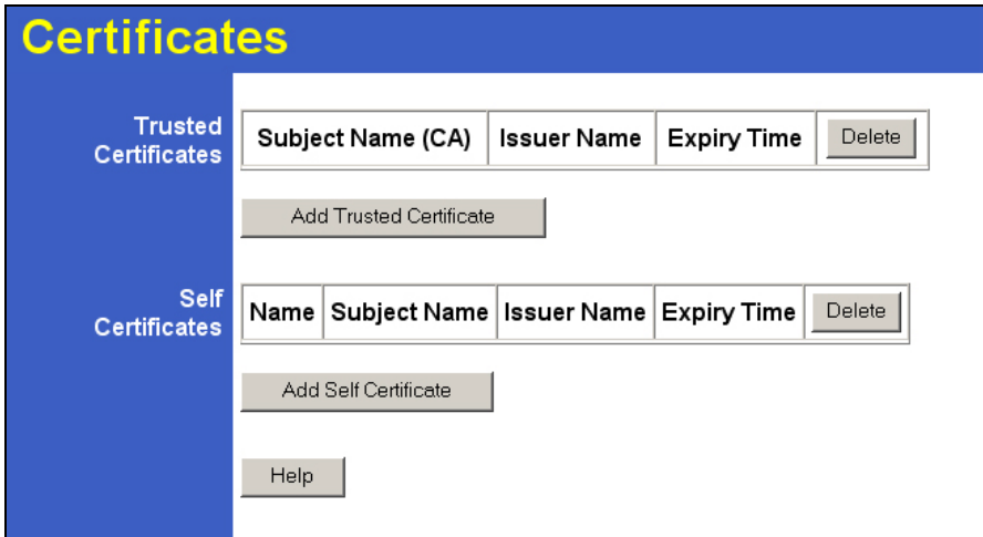
Figure 84: Certificates Screen
