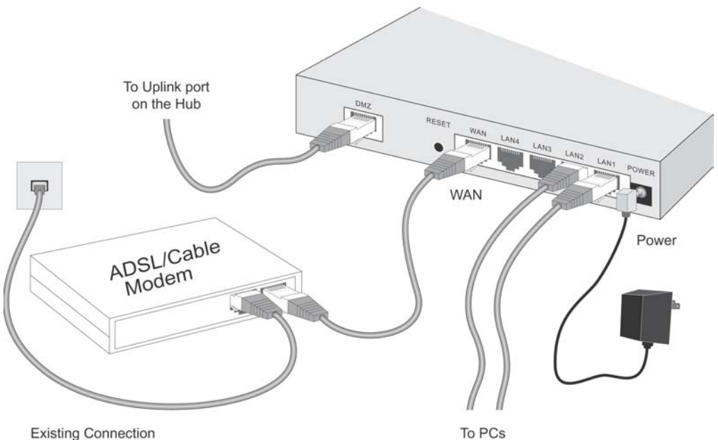
Figure 4: Installation Diagram
