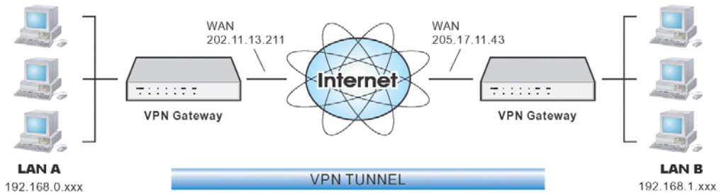
Figure 54: Connecting 2 TW100-BRV304s
