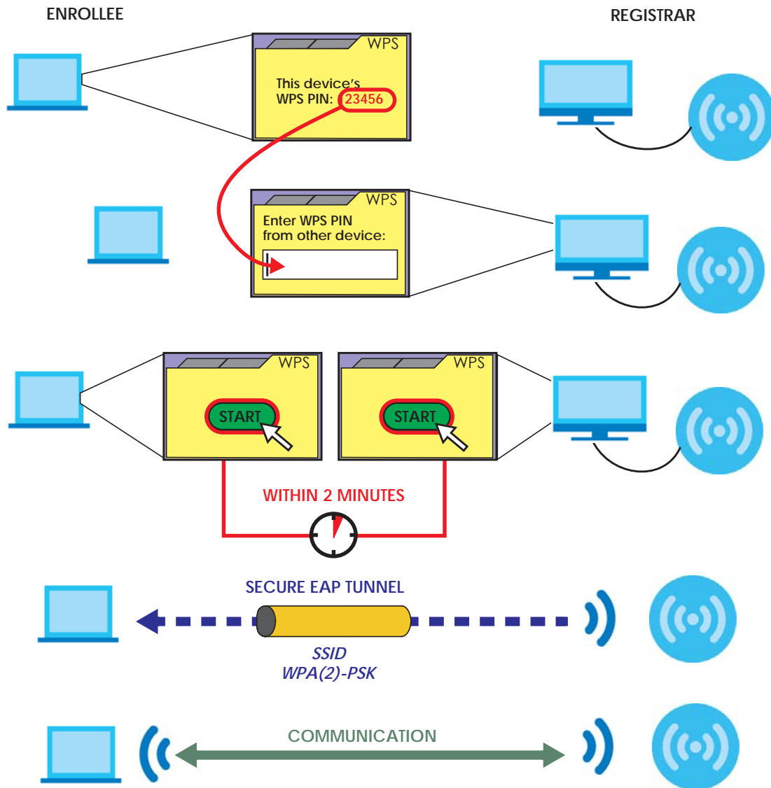
Figure 22 Example WPS Process: PIN Method
