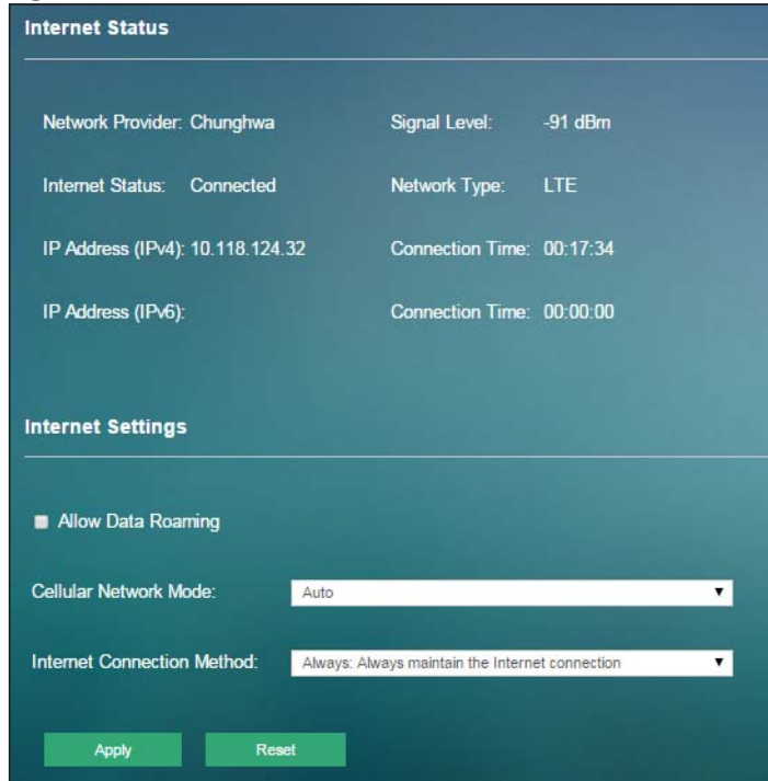
Figure 11 Internet > Internet Status
