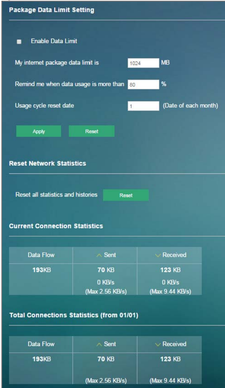
Figure 15 Internet > Data Usage/Statistic
