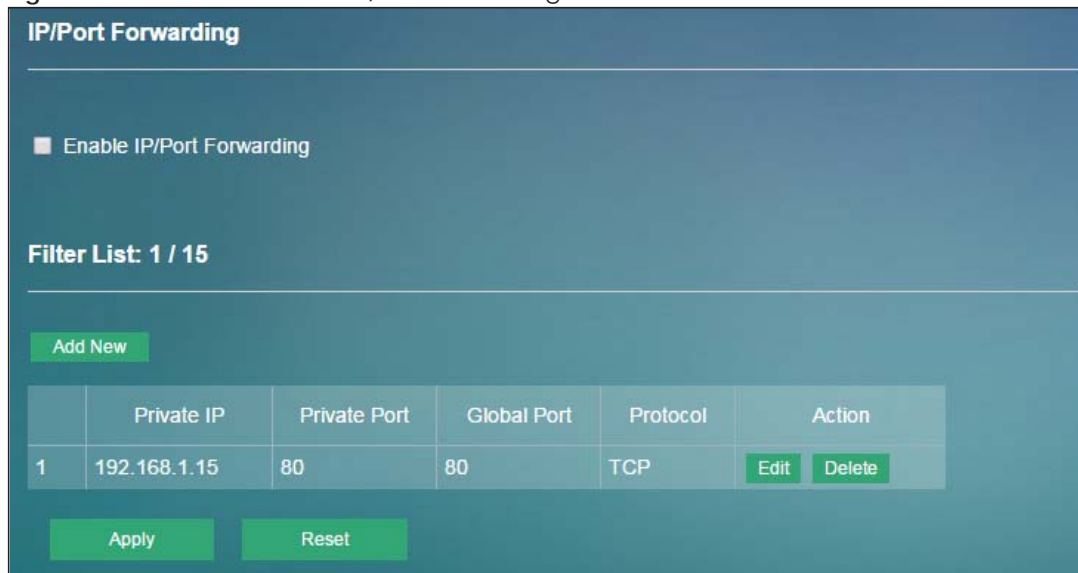
Figure 33 Router &gt; Firewall &gt; IP/Port Forwarding
