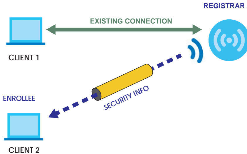
Figure 25 WPS: Example Network Step 2
