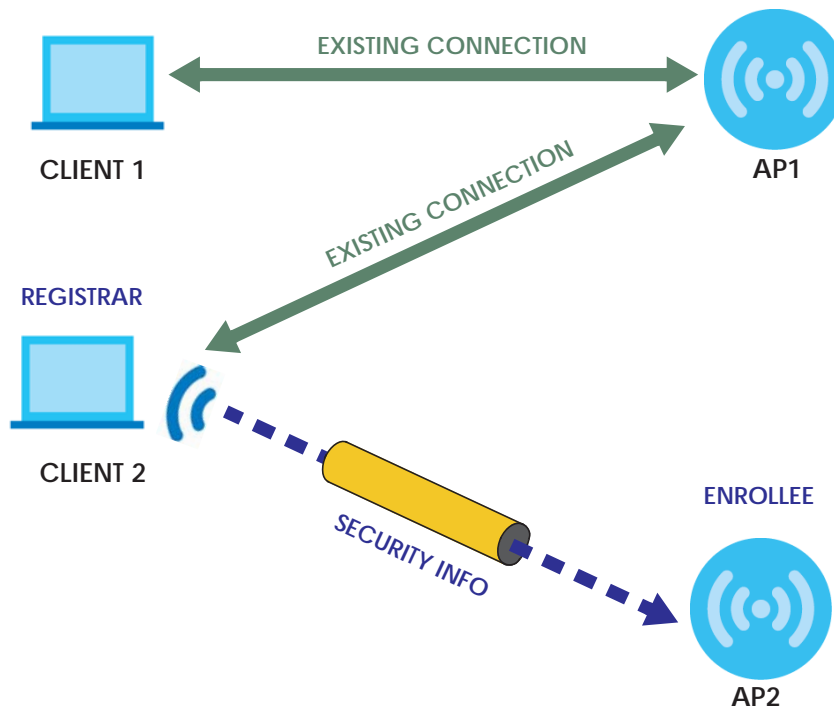
Figure 26 WPS: Example Network Step 3
