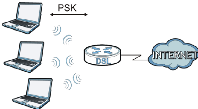
Figure 171 WPA(2)-PSK Authentication
