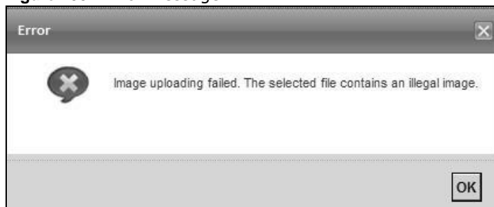
Figure 155 Error Message
