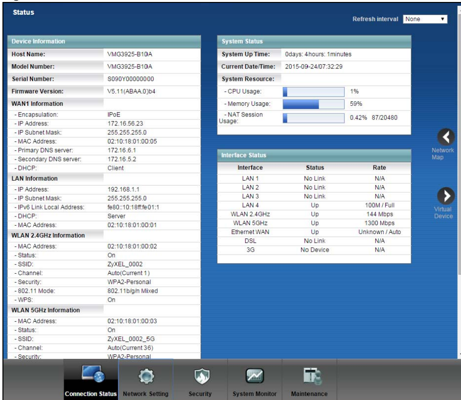
Figure 15 Status Screen
