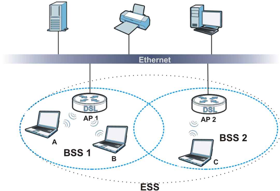
Figure 136 Infrastructure WLAN
