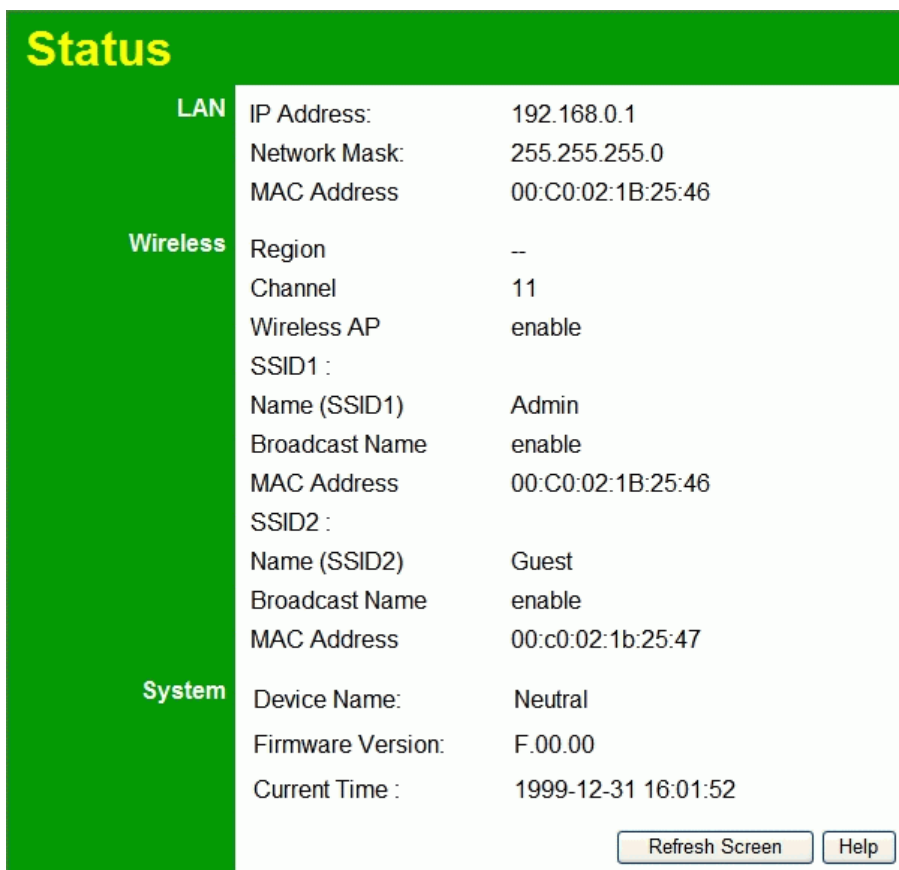
Figure 68: Status Screen - Bridge Mode
