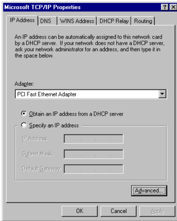
Figure 17: Windows NT4.0 - IP Address
