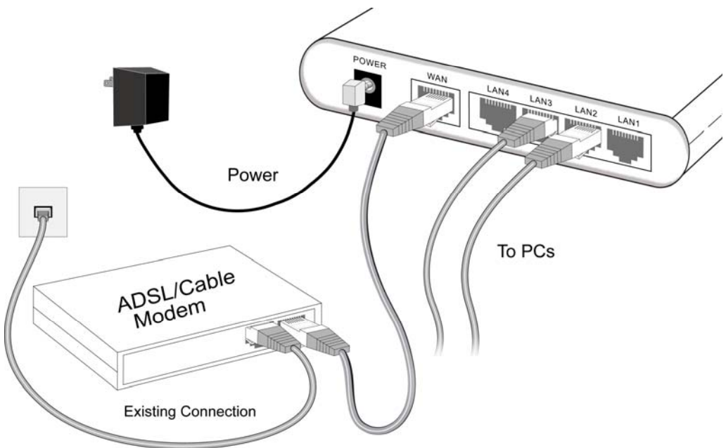
Figure 4: Installation Diagram
