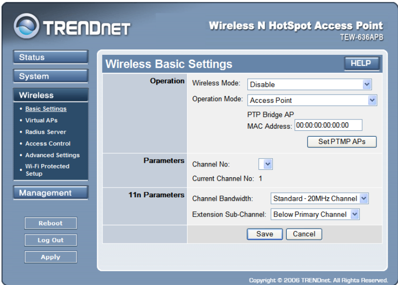
Figure 8: Wireless Basic Screen
