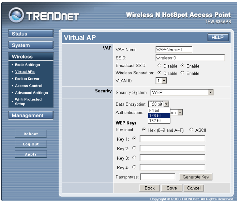
Figure 12: WEP Wireless Security Screen
