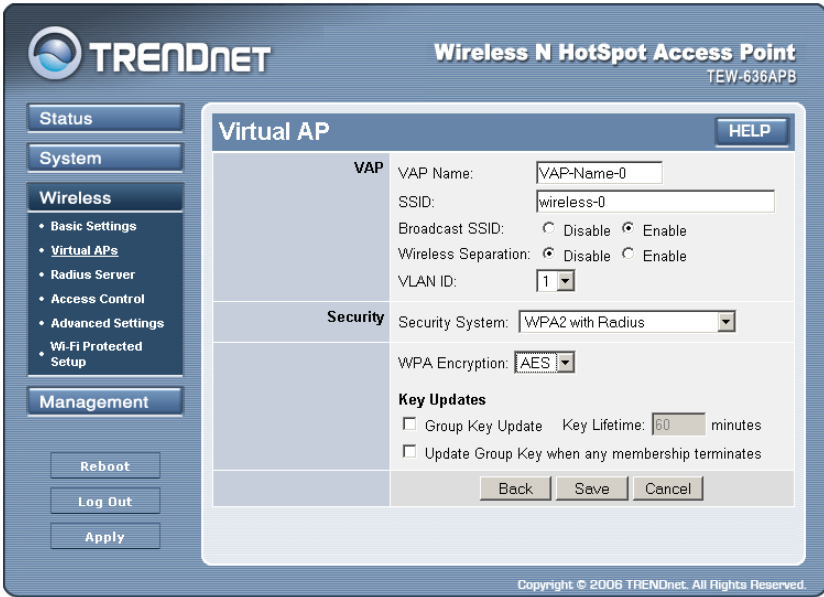
Figure 17: WPA2 with Radius Wireless Security Screen
