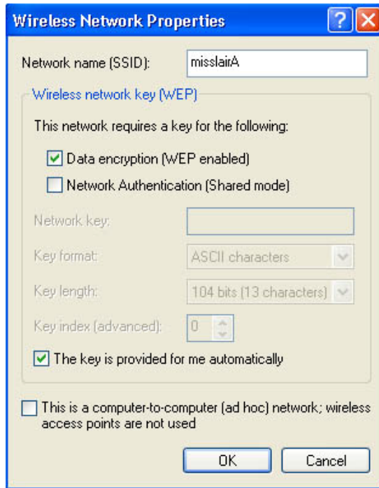
Figure 49: Properties Screen
