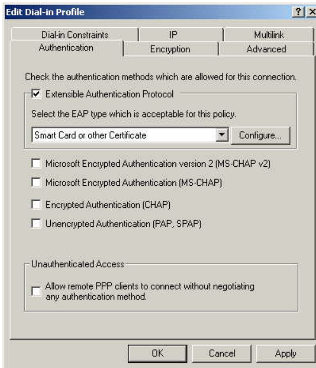
Figure 39: Authentication Screen
