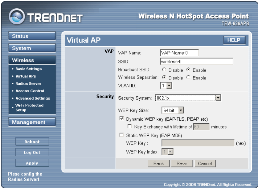
Figure 19: 802.1x Wireless Security Screen
