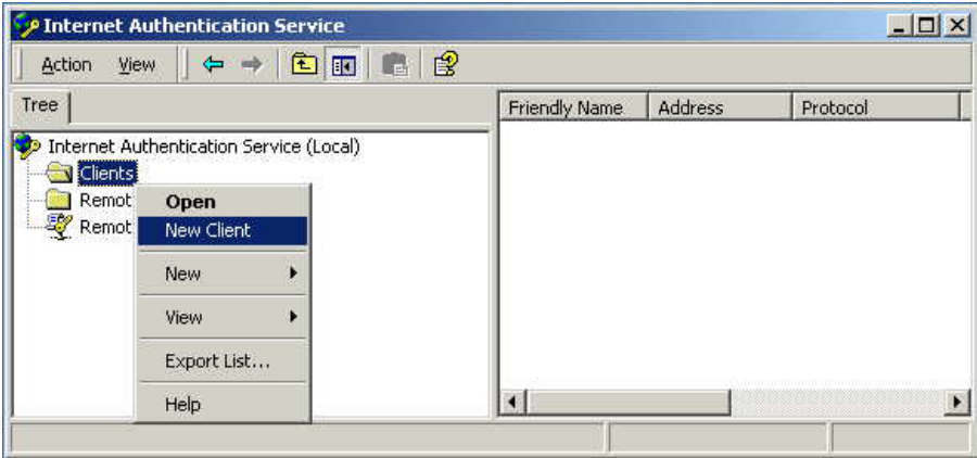
Figure 37: Service Screen
