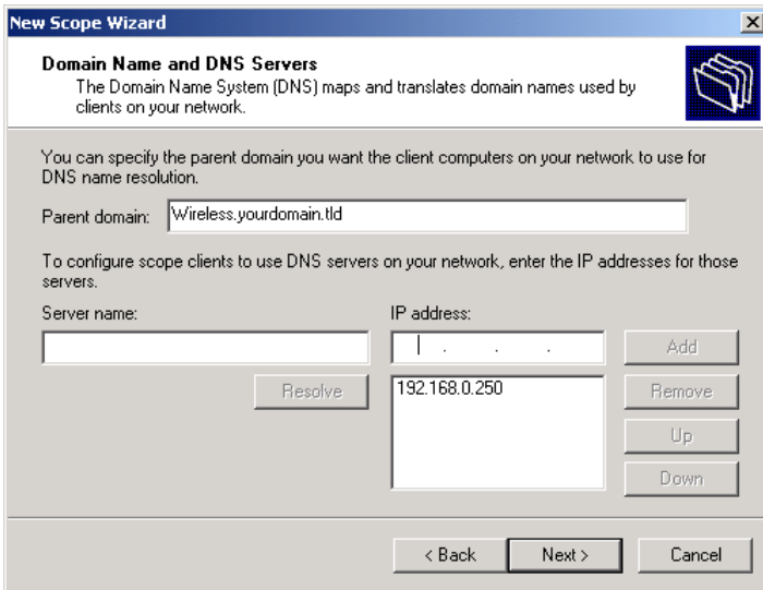
Figure 30: DNS Screen
