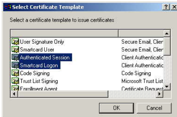
Figure 32: Template Screen
