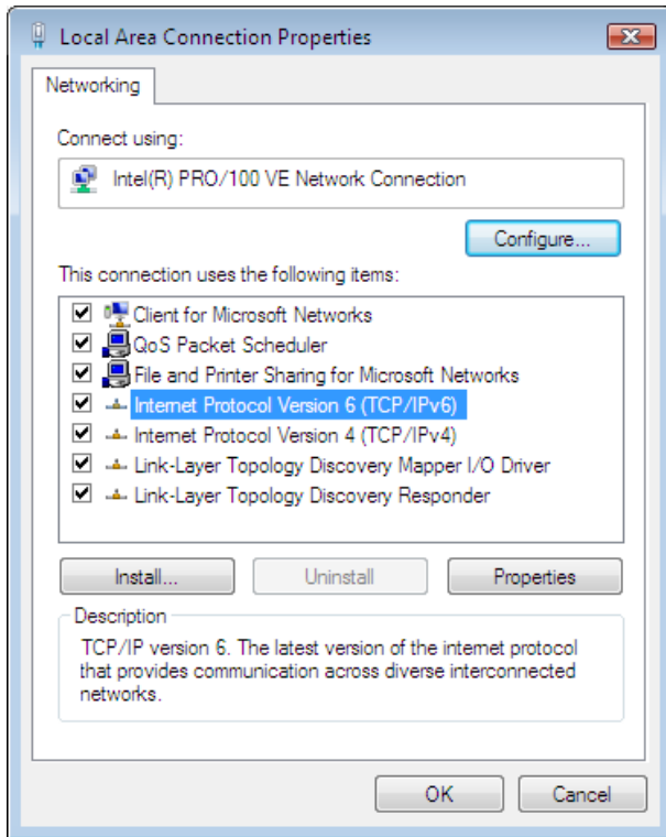
Figure 71: Network Configuration (Windows Vista)
