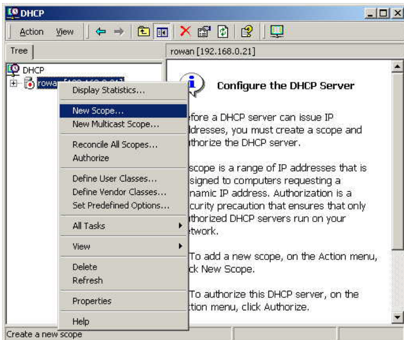
Figure 28: DHCP Screen
