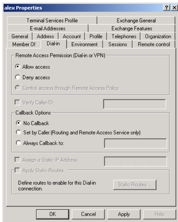
Figure 40: Dial-in Screen
