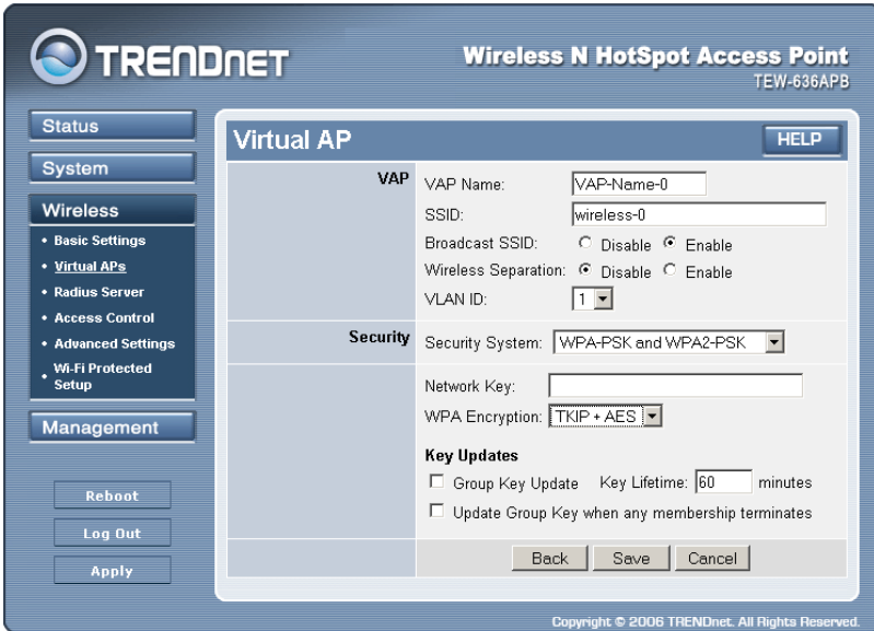
Figure 15: WPA-PSK and WPA2-PSK Wireless Security Screen
