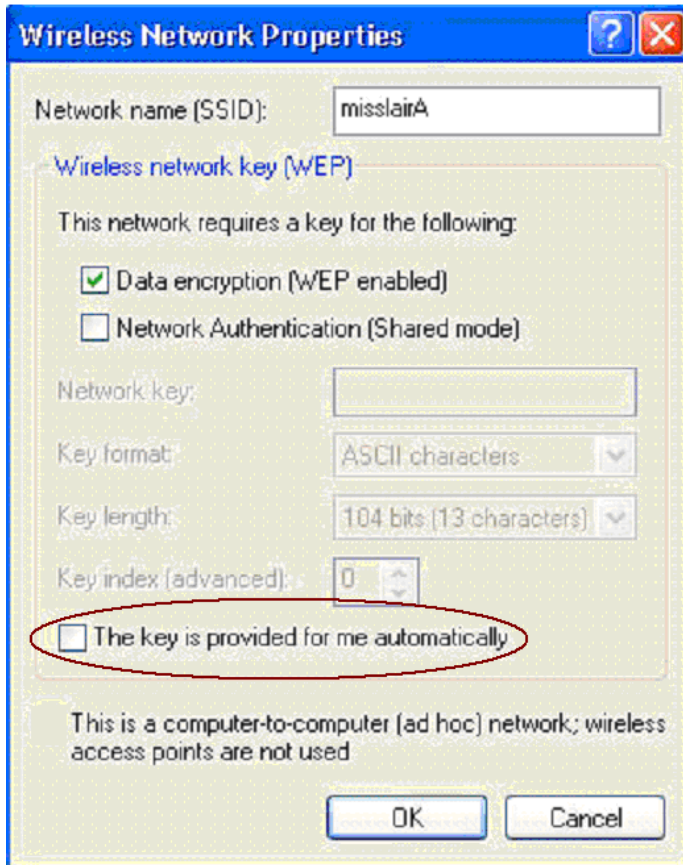
Figure 50: Properties Screen
