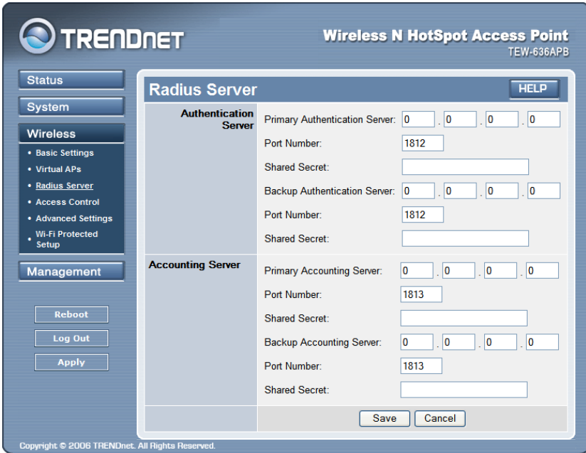
Figure 20: Advanced Settings
