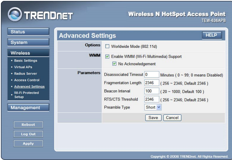
Figure 23: Advanced Settings
