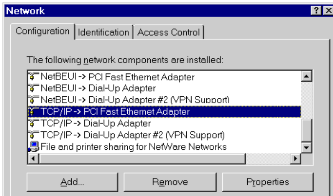
Figure 63: Network Configuration
