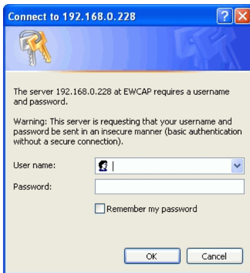
Figure 5: Password Dialog
