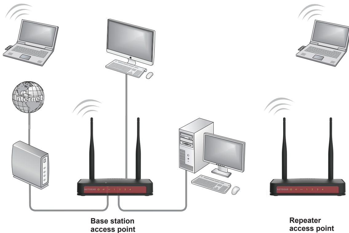
Figure 6. Wireless repeating scenario
