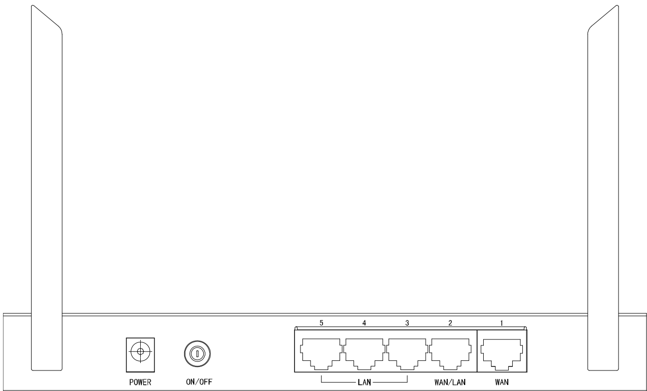
Figure 2-2 Rear Panel
