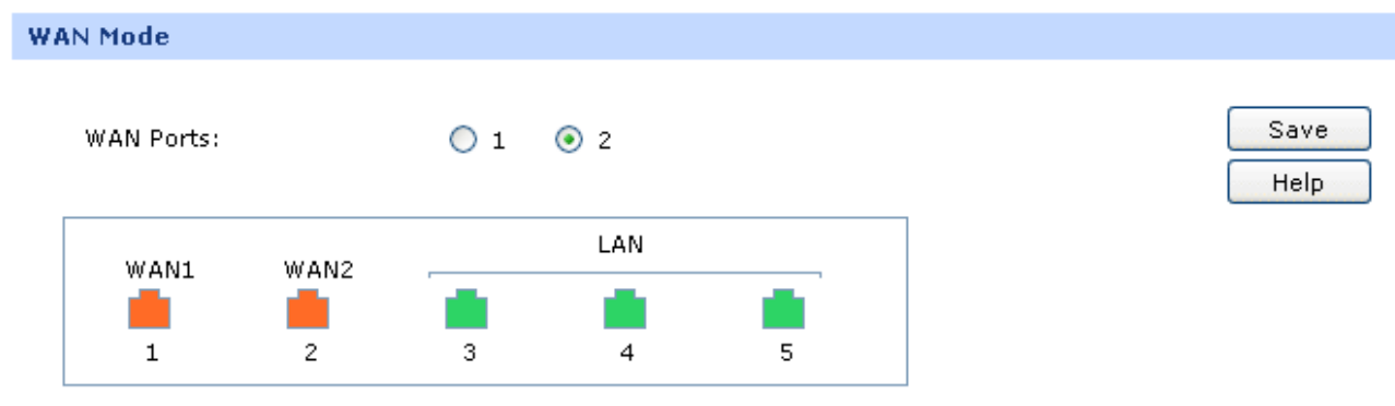
Figure 3-6 WAN Mode
