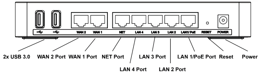
Figure 2: GWN7000 Back View
