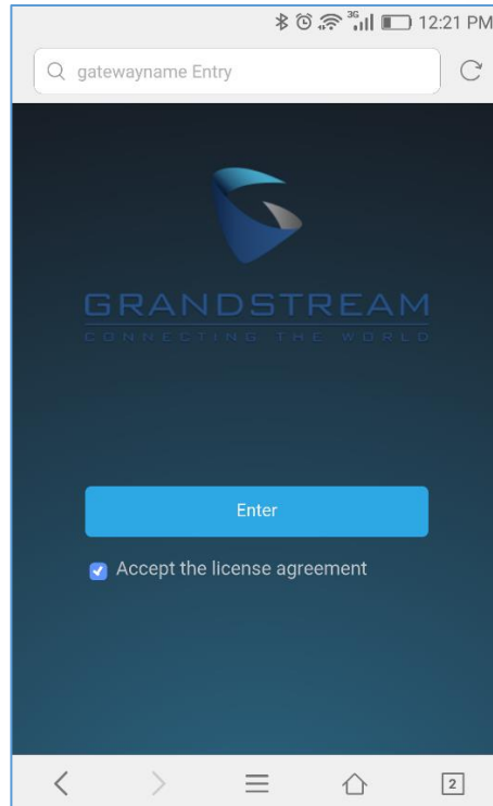
Figure 56: portal_default.html page
