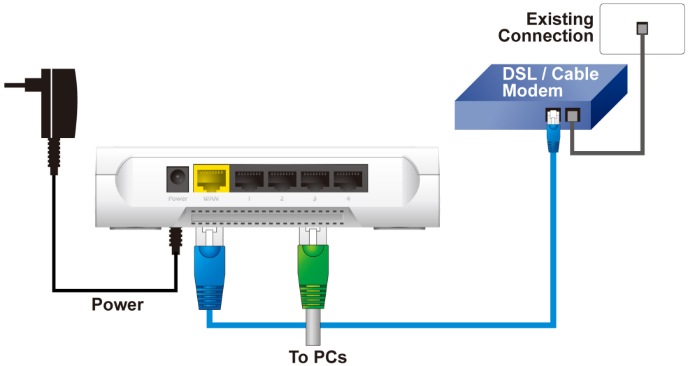
Figure 4: Installation Diagram
