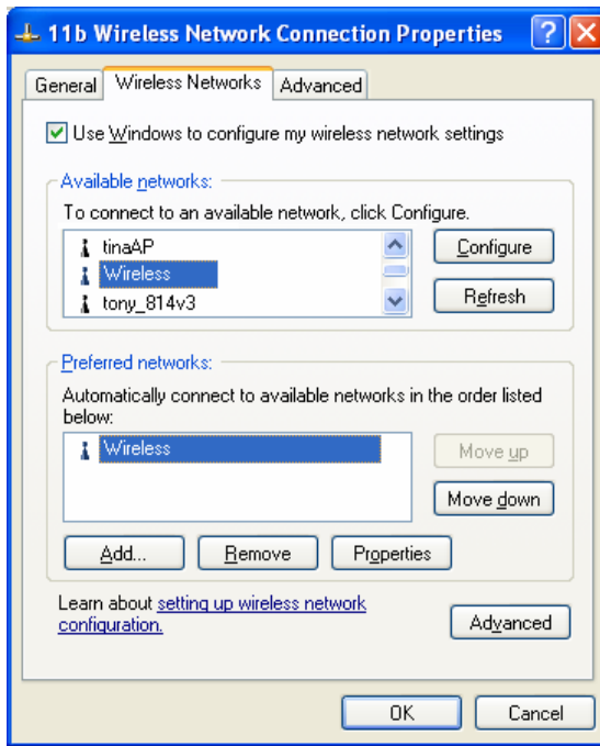
Figure 32: Preferred Networks
