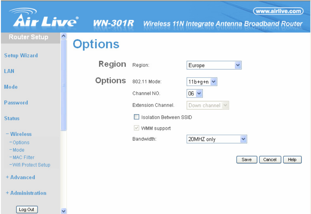
Figure 8: Wireless Screen
