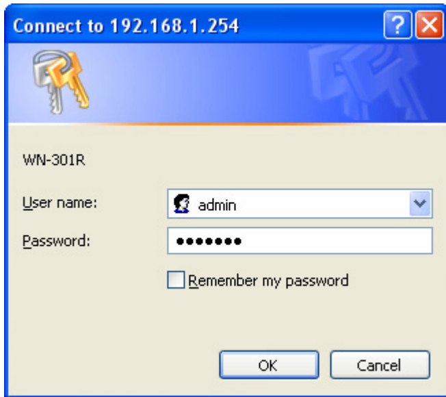
Figure 15: Password Dialog
