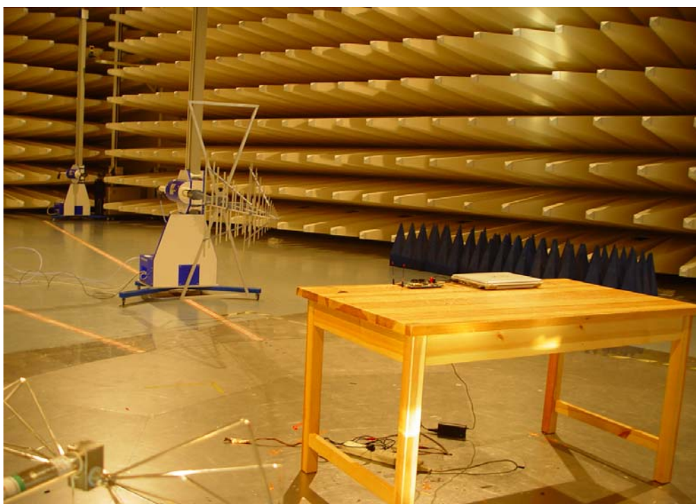
Receiver Spurious Emission Test Setup
