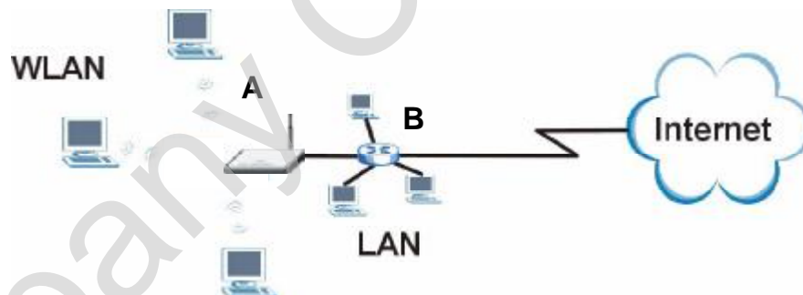
Figure 24 Wireless Internet Access in AP Mode
