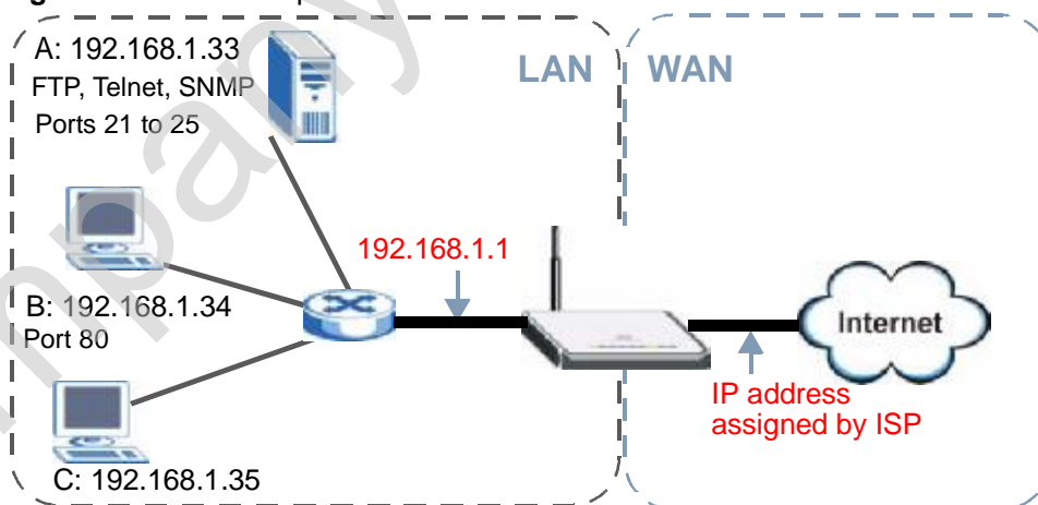
Figure 65 NAT Example
