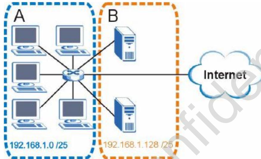
Figure 126 Subnetting Example: After Subnetting
