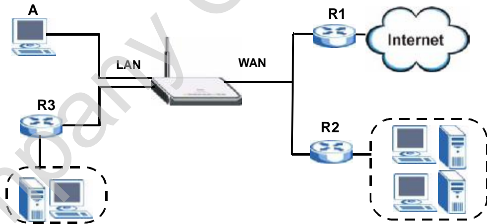
Figure 77 Example of Static Routing Topology
