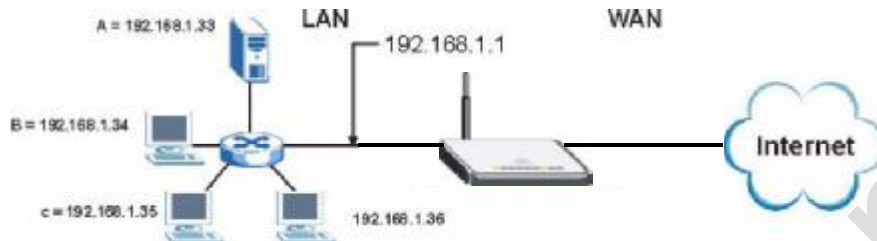
Figure 70 Multiple Servers Behind NAT Example
