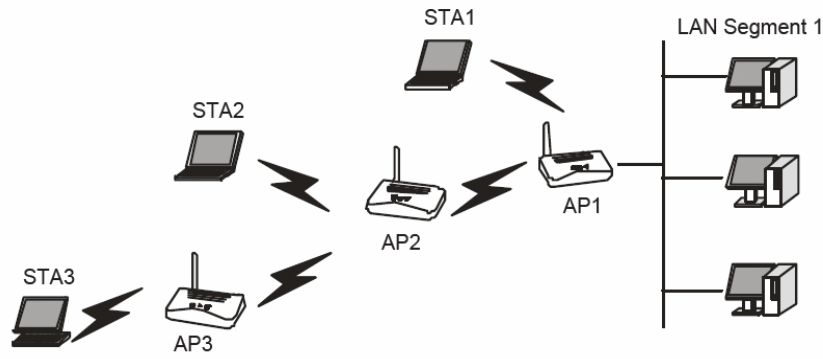
Figure 4-8 Wireless repeating
