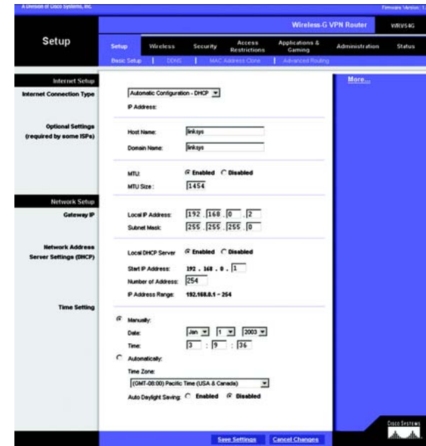
Figure 6-2: Setup Tab/DHCP Internet Connection Type
