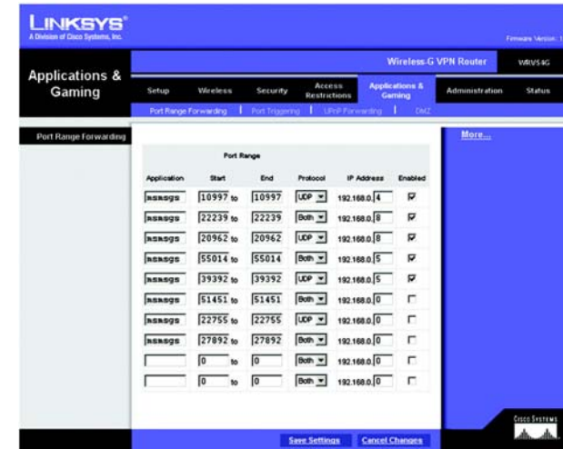
Figure 6-26: Port Range Forwarding
