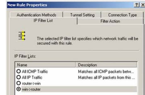
Figure C-10: IP Filter List Tab
