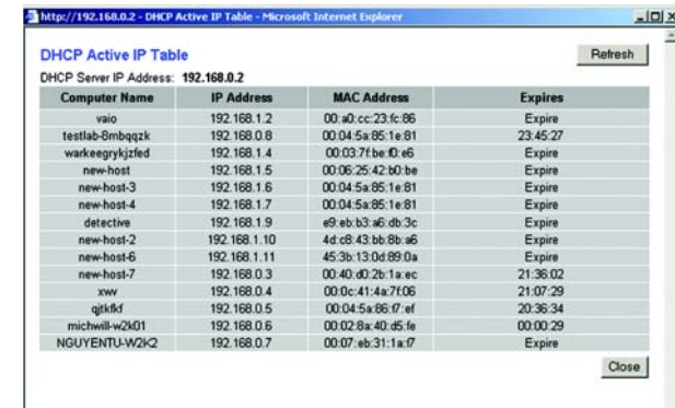
Figure 6-37: DHCP Active IP Table
