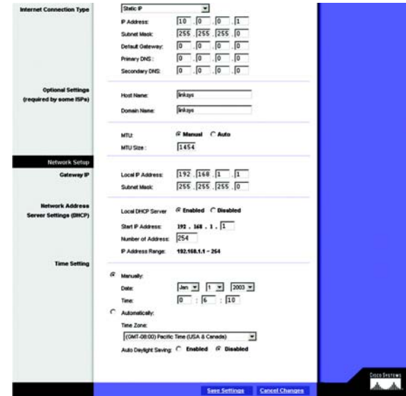
Figure 6-3: Static Internet Connection Type
