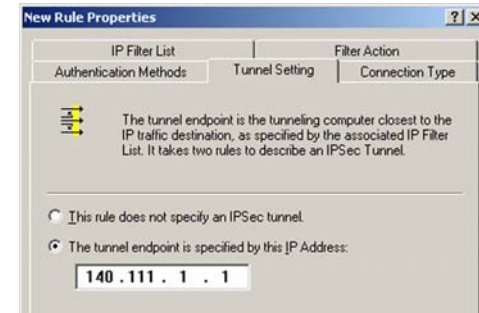
Figure C-16: Tunnel Setting Tab
