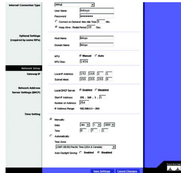
Figure 6-4: PPPoE Internet Connection Type
