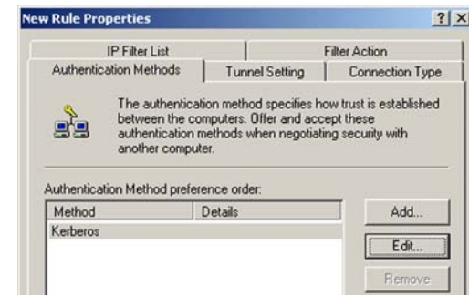
Figure C-21: Authentication Methods Tab
