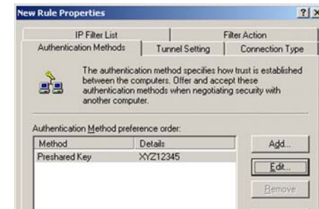
Figure C-15: New Preshared Key
