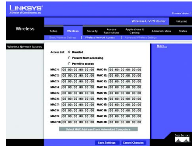
Figure 6-13: Wireless Network Access
