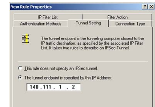
Figure C-24: Tunnel Setting Tab
