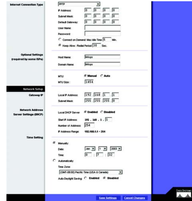
Figure 6-5: PPTP Internet Connection Type
