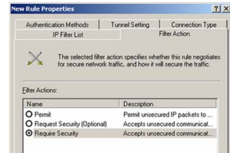
Figure C-11: Filter Action Tab
