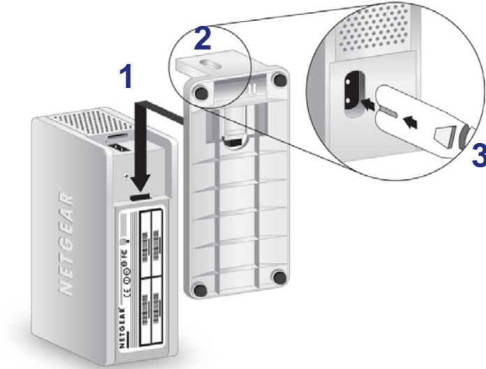
Figure 6. Attach the stand and the power adapter cord.
