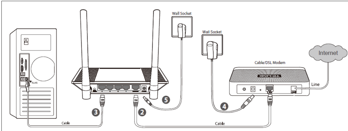
Figure 2-1 Hardware Installation of the 300Mbps High Power Router
