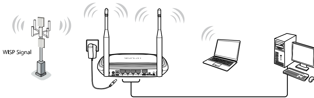
Figure 2-1 Hardware Installation of the TL-WR843ND in WISP Client Router mode
