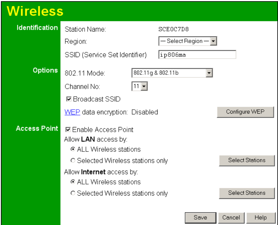
Figure 7: Wireless Screen
