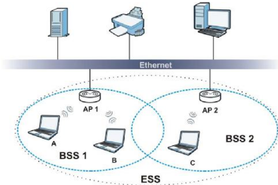
Figure 110 Infrastructure WLAN
