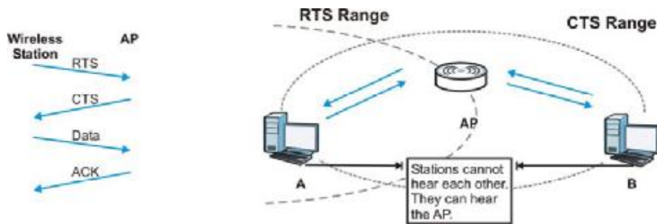
Figure 111 RTS/CTS
