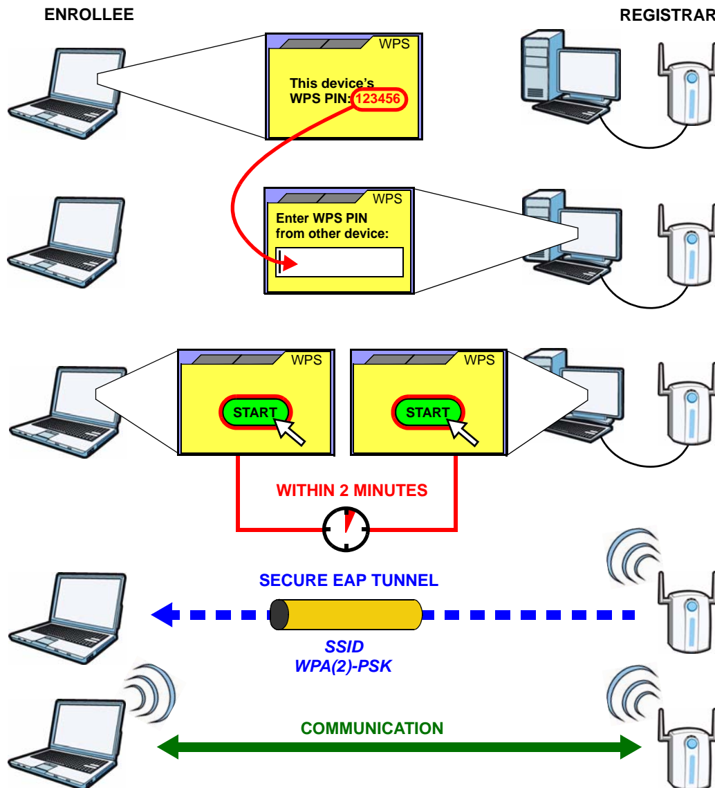
Figure 23 Example WPS Process: PIN Method
