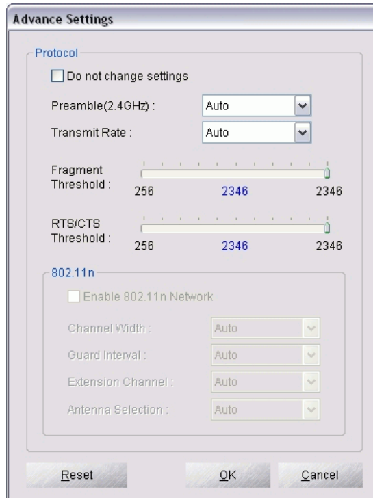
Figure 9: Advanced Settings Screen
