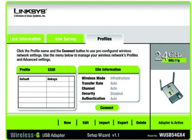
Figure 5-9: Profiles Screen
