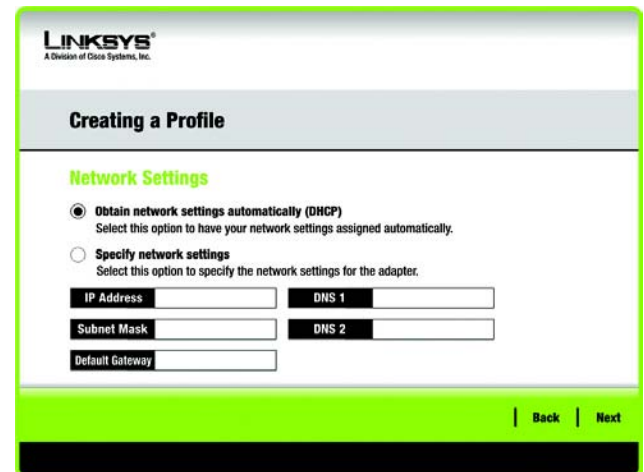
Figure 5-14: Network Settings
