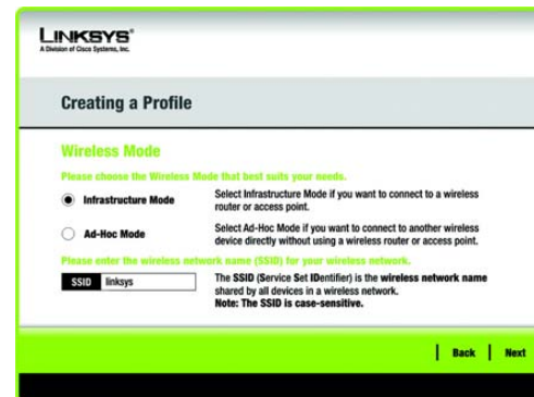
Figure 4-11: Wireless Mode
