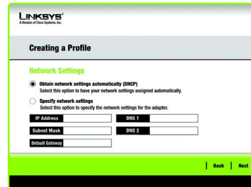
Figure 4-10: Network Settings
