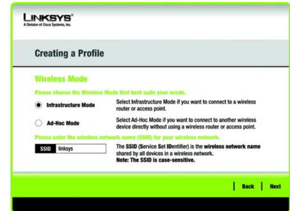
Figure 5-15: Wireless Mode
