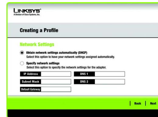
Figure 4-6: Network Settings
