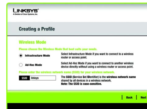
Figure 4-7: Wireless Mode
